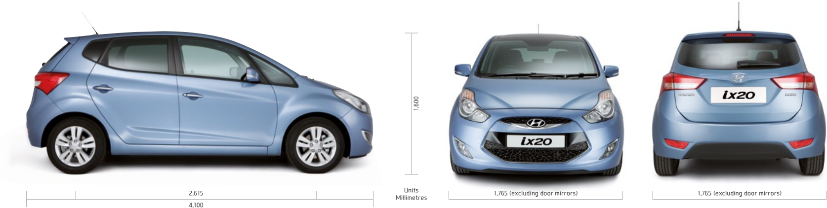
ix20 DIMENSIONS
